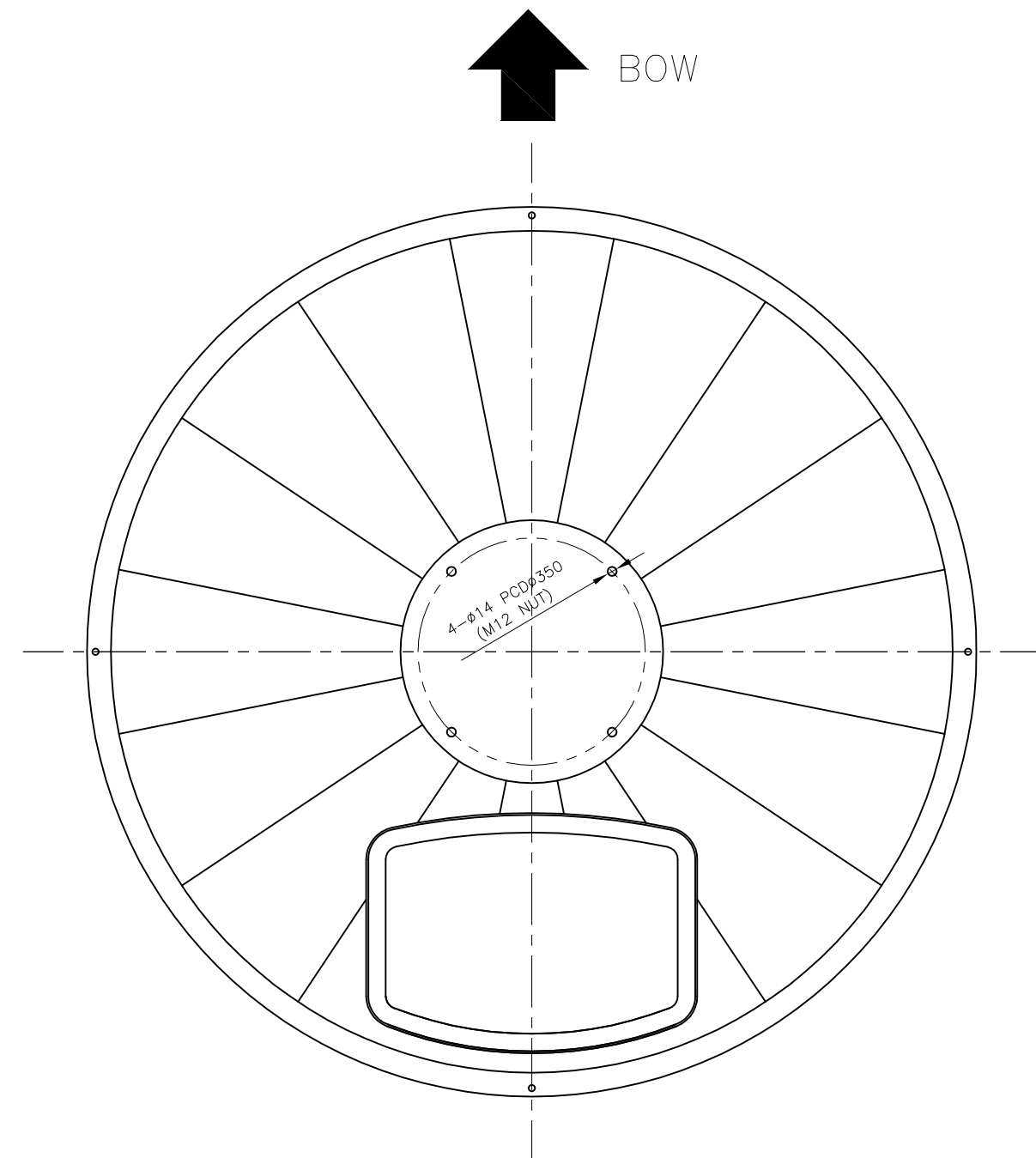
MOUNTING SURFACE PATTERN (BOTTOM VIEW)
